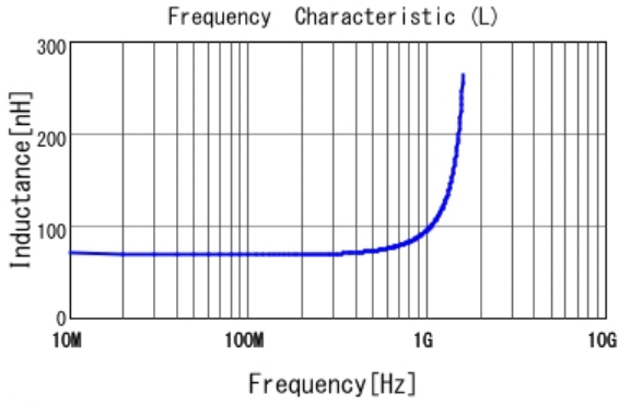
■ LQW2BAS68NJ00 L
