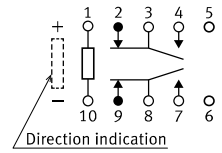
Schematic (BOTTOM VIEW) Single side stable (De-energize)
