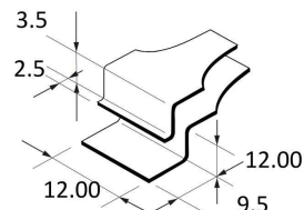
Dimensions mm
