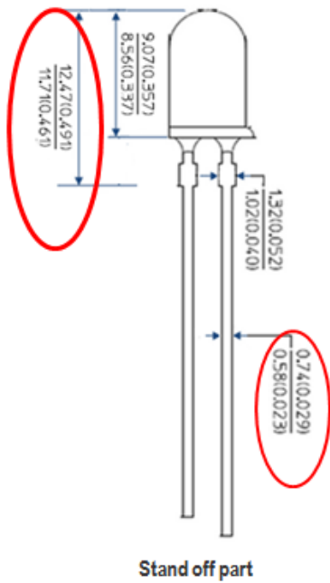
Existing 25mils leadframe
