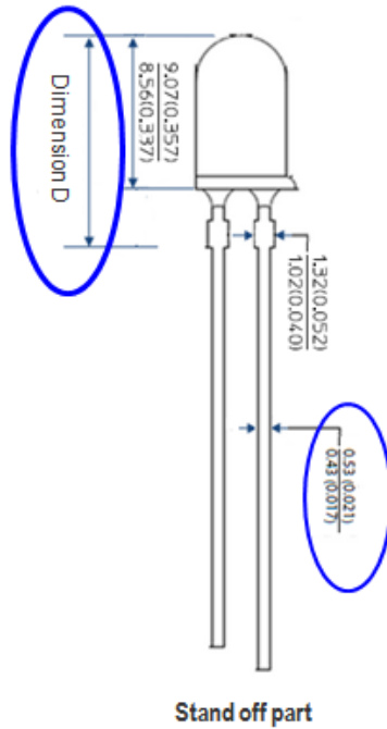
18mils leadframe
