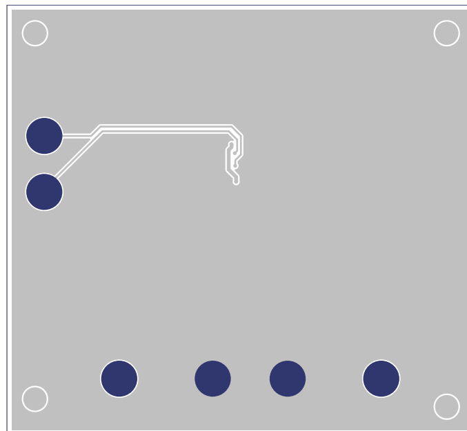
Figure 4: Bottom Layer
