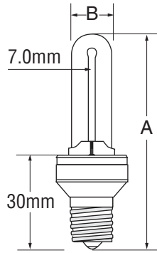
E17 Base GTL3 Replacement w/Ballast
