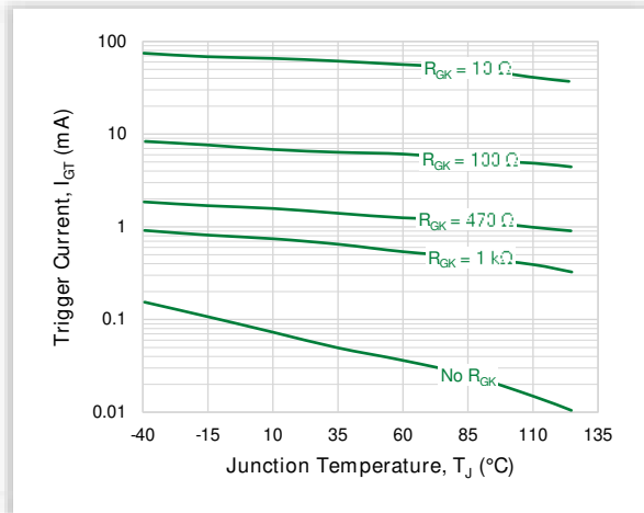
Figure 7. Typical DC Gate Trigger Current with R_GK vs. Junction Temperature for S6X8xS
