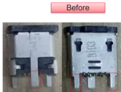
No dimples on shell soldering tail
