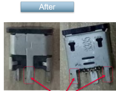
Add dimples to each of shell soldering tails
