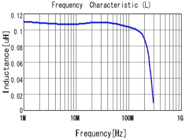
■ LQM2MPZR10MJH L
