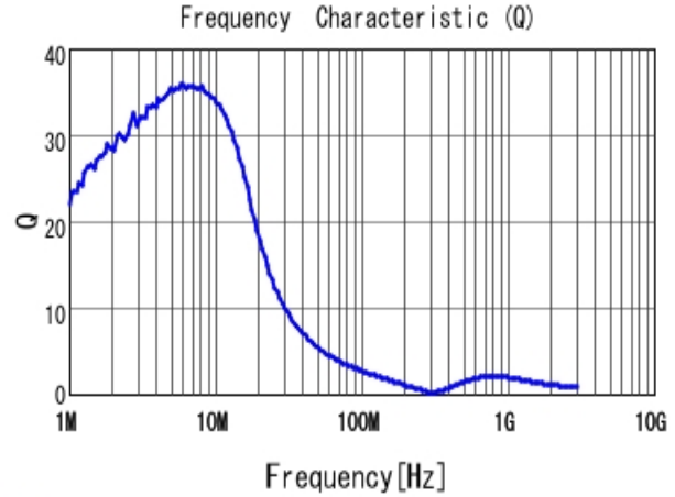
■ LQM2MPZR10MJH Q
