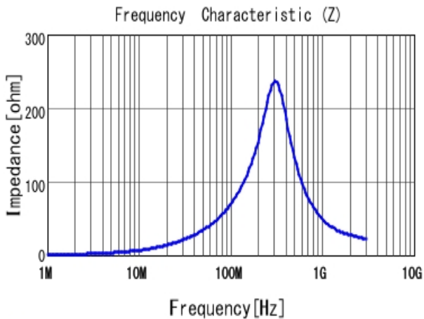
■ LQM2MPZR10MJH |Z|
