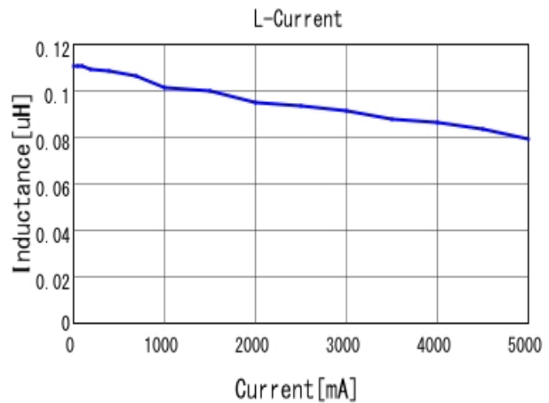
■ LQM2MPZR10MJH L-Current 20degC
