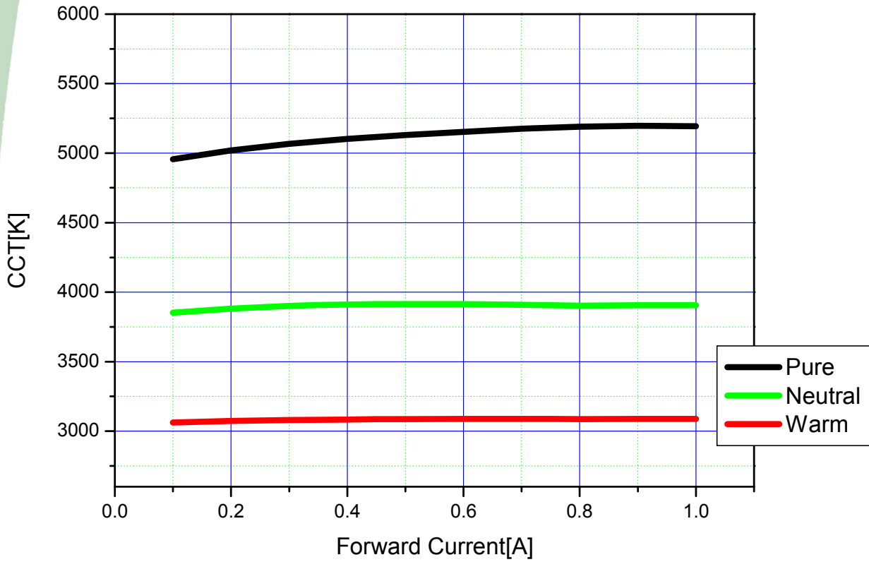
CCT vs. Forward Current, Ta=25°C
