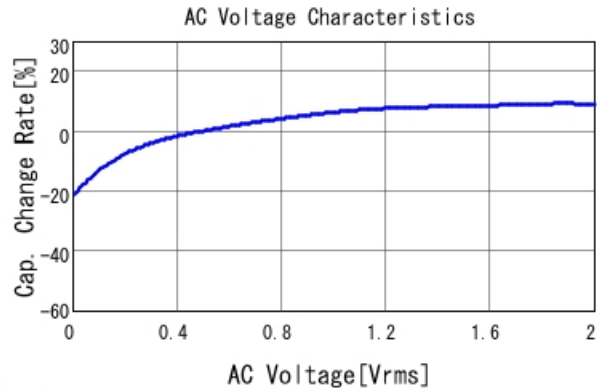
■ KRM21FR61E226MFA1 C-AC Voltage capchange, DCOV, 25.0d
