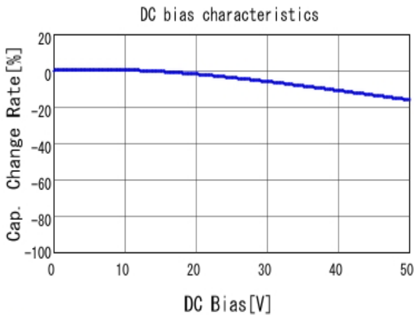
■ GCJ188R91H472KA01 C-DC bias capchange, 25.0degC, AC1.
