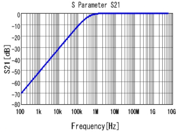
■ GCJ188R91H472KA01 S21 DC0V, 25degC
