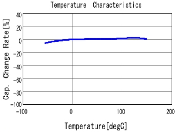
■ GCJ188R91H472KA01 C-Temp. capchange, DC0.0V, AC1.0V r m
