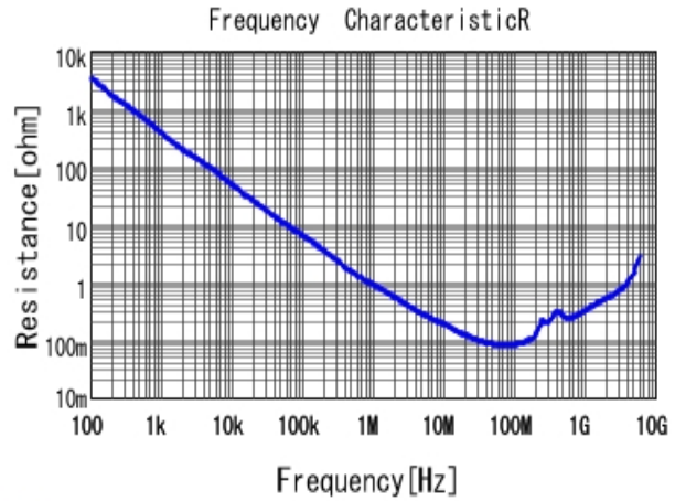
■ GCJ188R91H472KA01 R DCOV, 25degC
