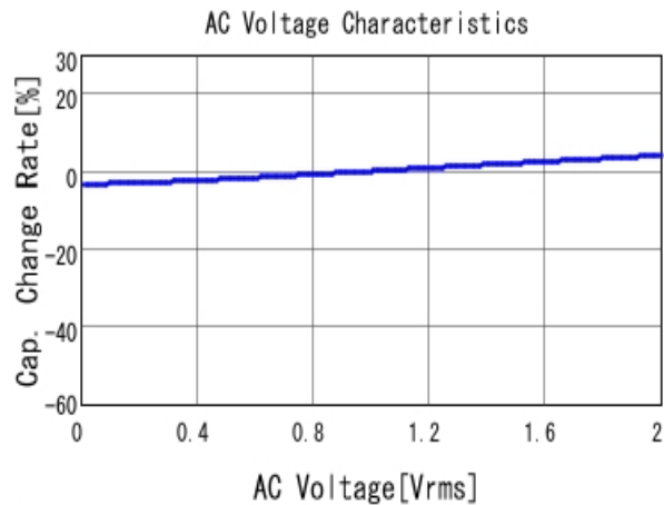
■ GCJ188R91H472KA01 C-AC Voltage capchange, DCOV, 25.0d
