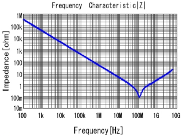
■ GCJ188R91H472KA01 |Z| DCOV, 25degC
