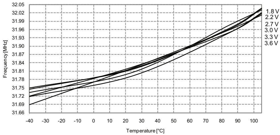
Figure 37-329. 32MHz internal oscillator frequency vs. temperature DFLL enabled, from the 32.768kHz internal oscillator
