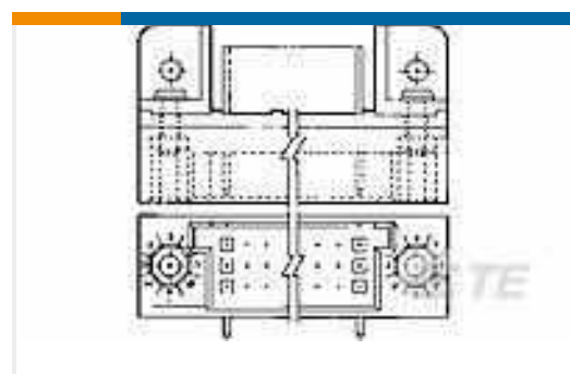
TE Teilenummer533288-7 HDI PIN ASSY 3 ROW 150 POS R/A
