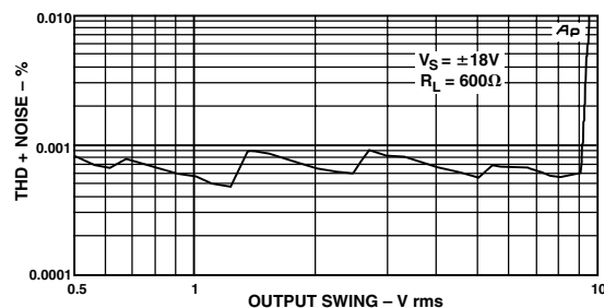
Figure 4. Headroom, THD + Noise vs. Output Amplitude ( \text{V rms} ); R_{LOAD} = 600\ \Omega , V_{SUP} = \pm 18\ \text{V}
