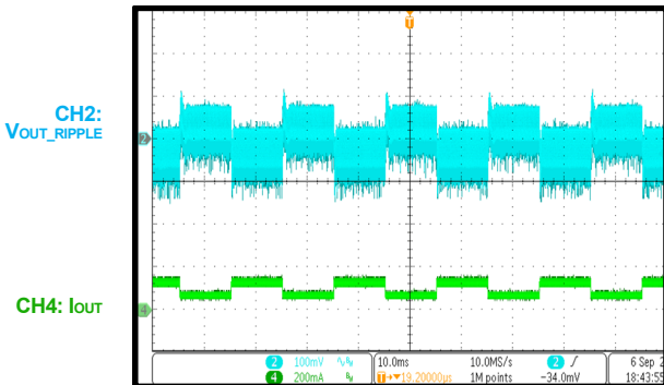
Load Transient
