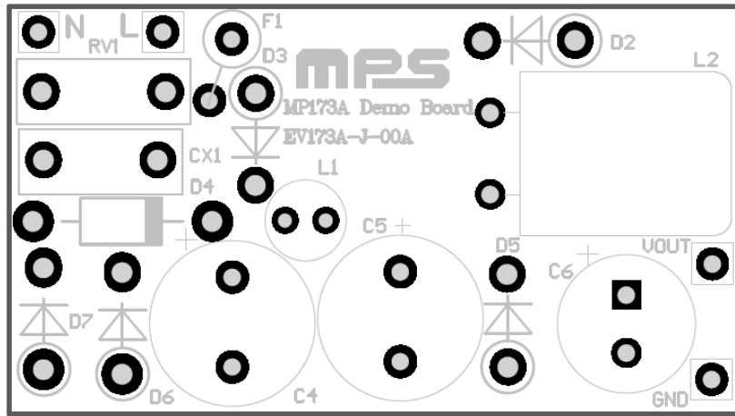
Figure 2: Top Layer
