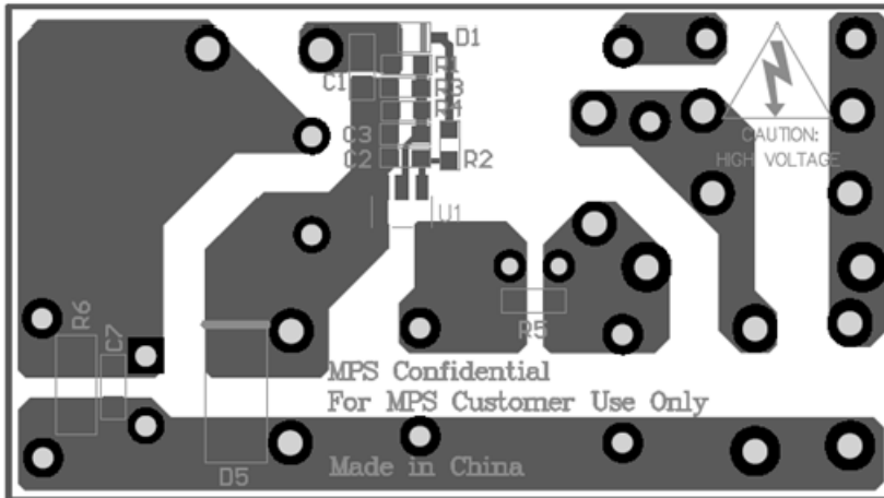
Figure 3: Bottom Layer
