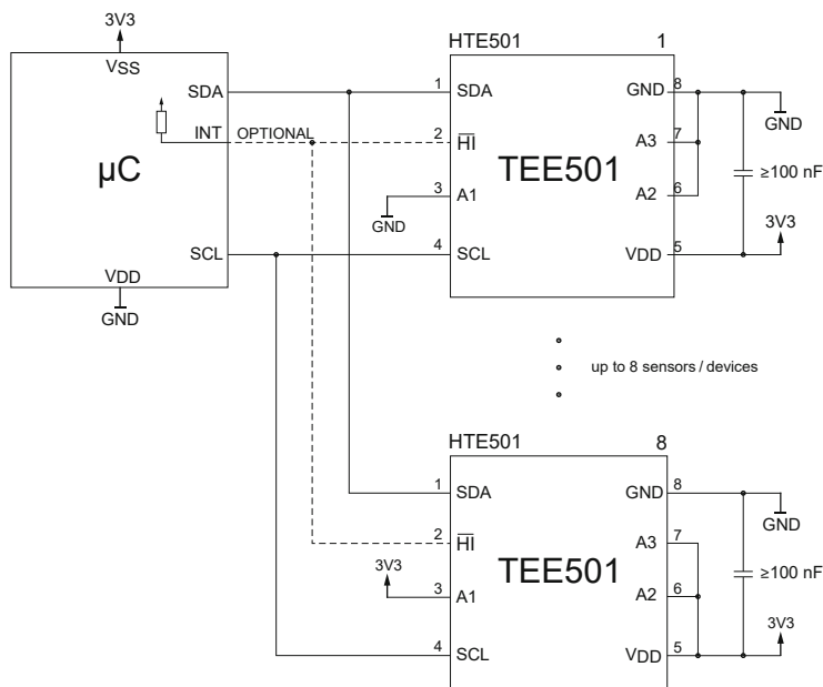
Figure 2: Typical application schematic
