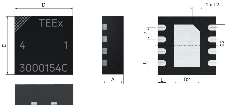
Figure 22: Package layout
