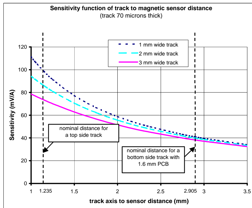
Figure 11: Sensitivity (mV/A) versus track width and versus distance between the track and the Minisens sensing elements
