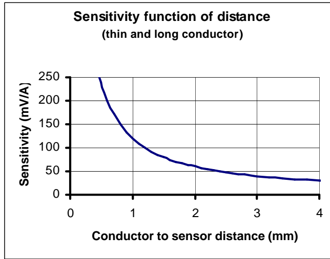
Figure 9: Sensitivity versus the distance between the conductor and the Minisens sensing elements
