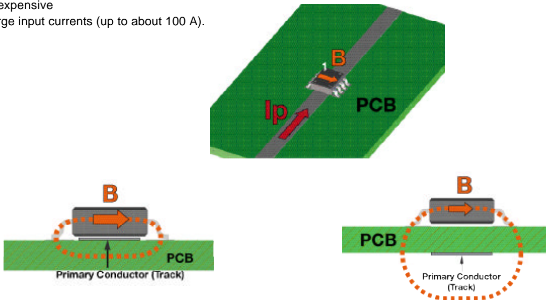
Figure 10: Principle of Minisens used to measure current in a PCB track
