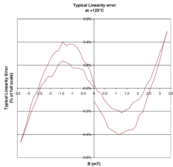
Figure 3: Typical linearity error at +125°C
