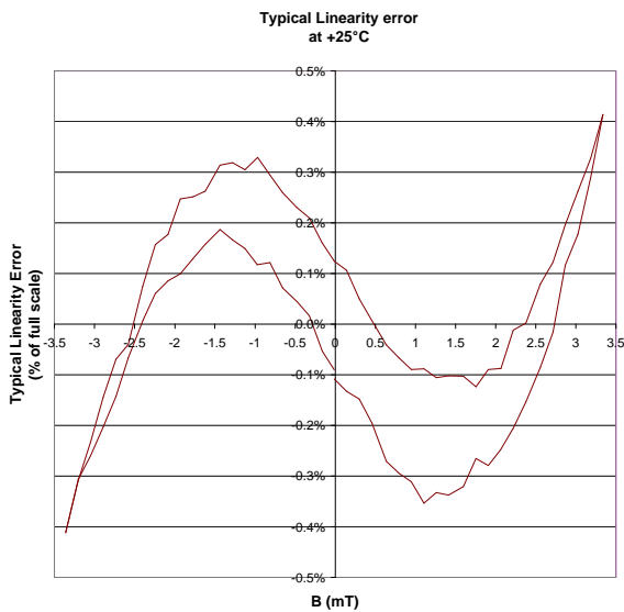
Figure 2: Typical linearity error at +25°C
