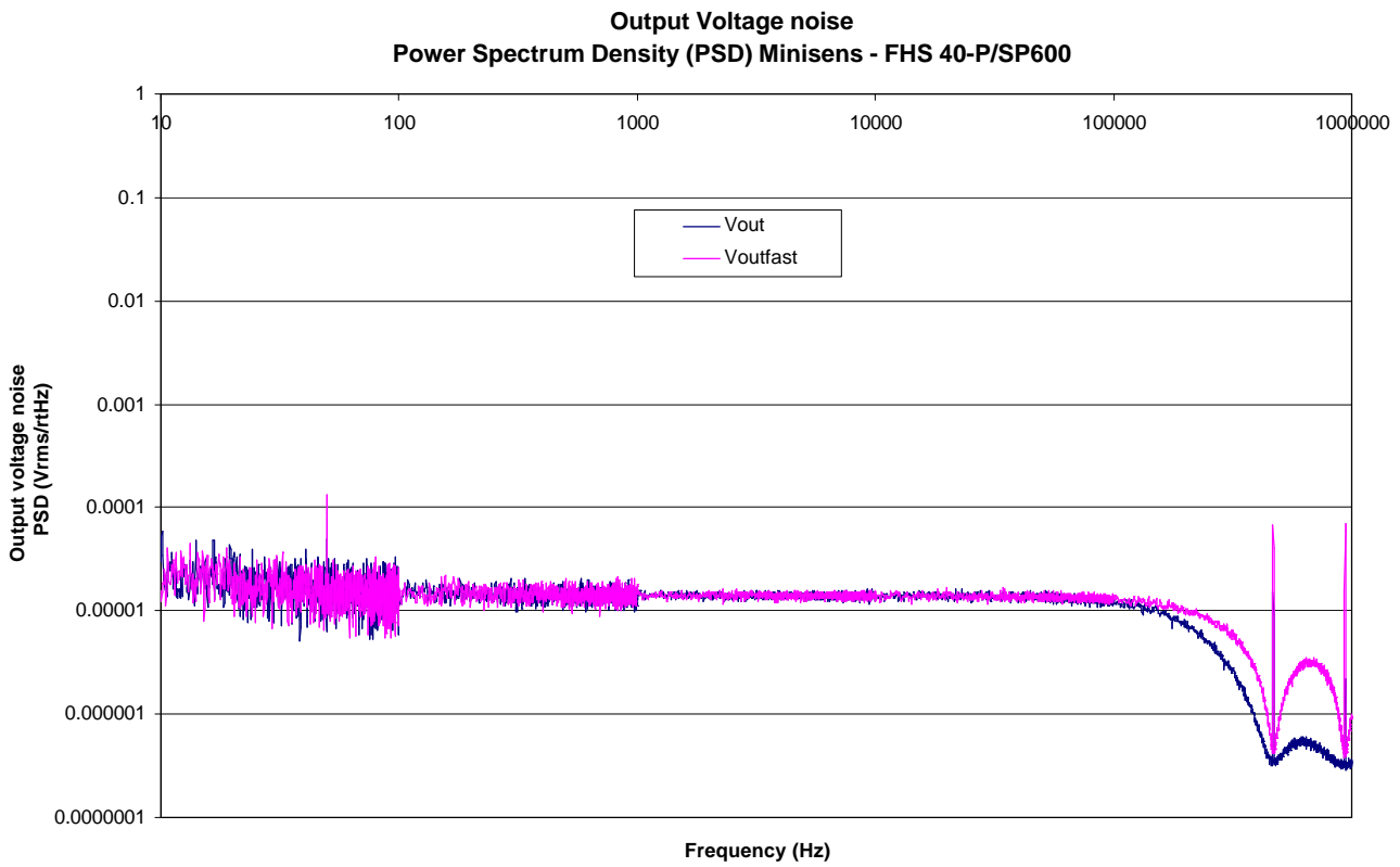
Figure 1: Output Voltage Noise
