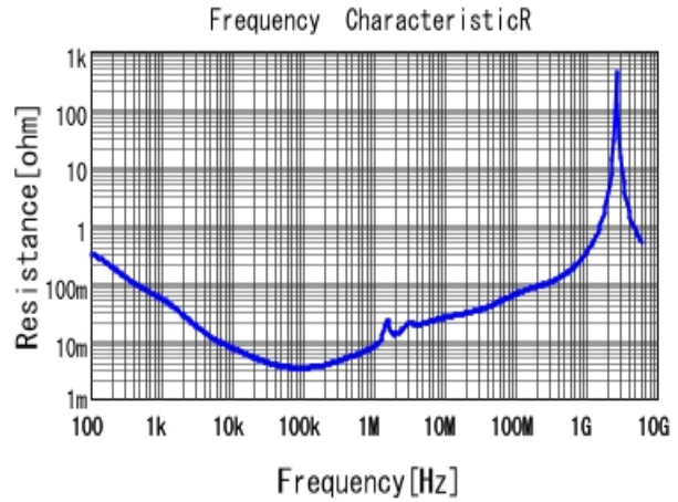
■ KCM55WR71J226MH01 R DCOV, 25degC
