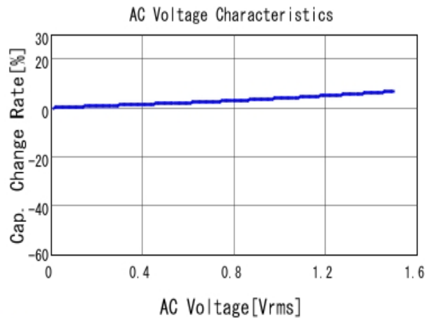
■ KCM55WR71J226MH01 C-AC Voltage capchange, DCOV, 25.0d
