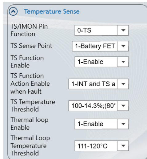
Figure 17: Temperature-Sense Settings
