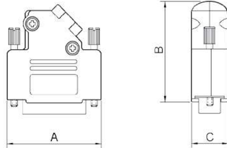
D-Sub-Hood
