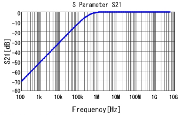
■ GRM155R71H472KA01 S21 DCOV, 25degC
