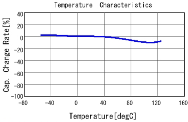
■ GRM155R71H472KA01 C-Temp. capchange, DCO. 0V, AC1. 0V rm
