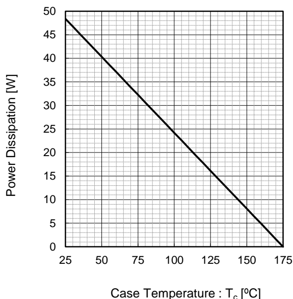
Fig.6 Power Dissipation
