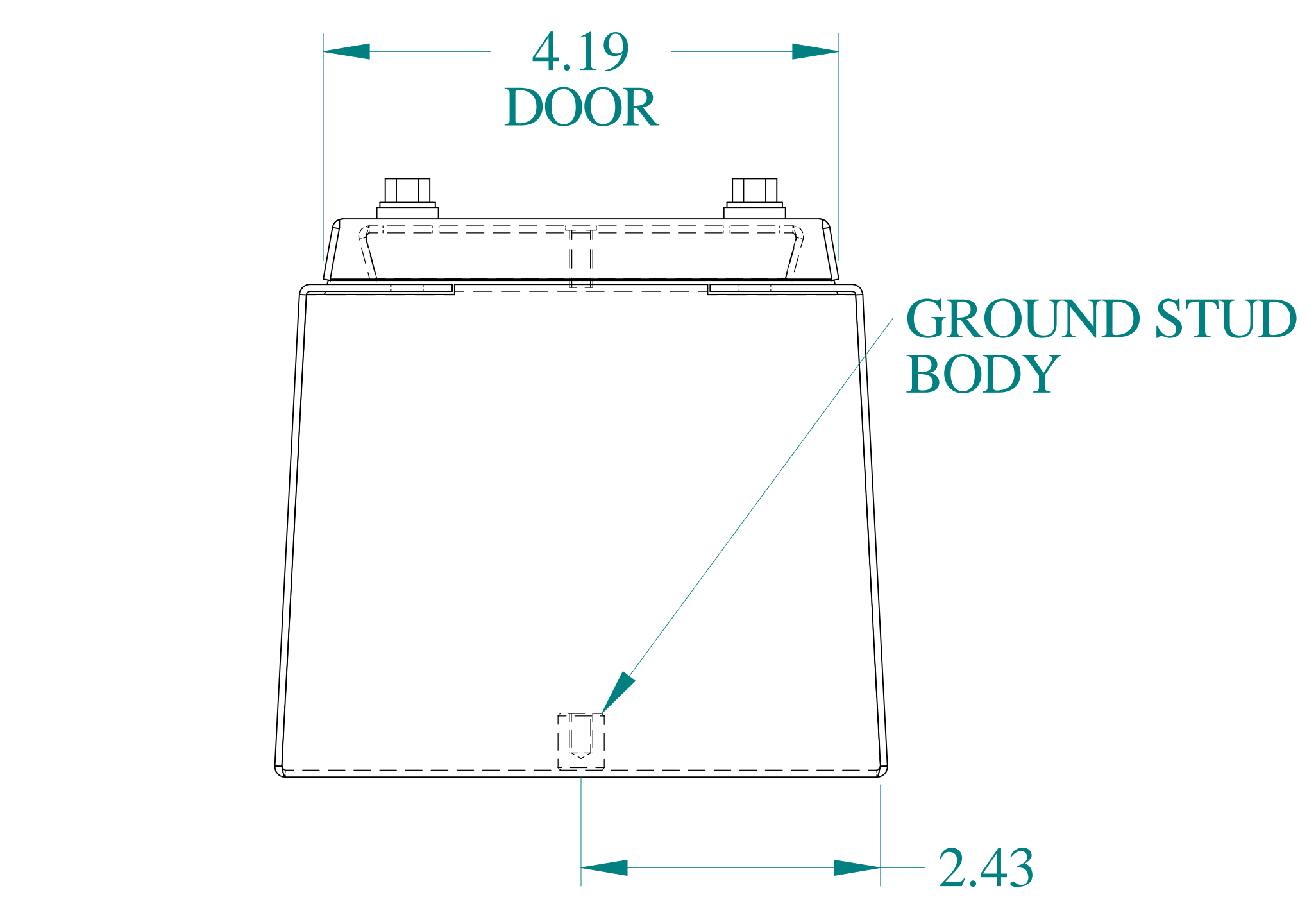
BOTTOM VIEW
