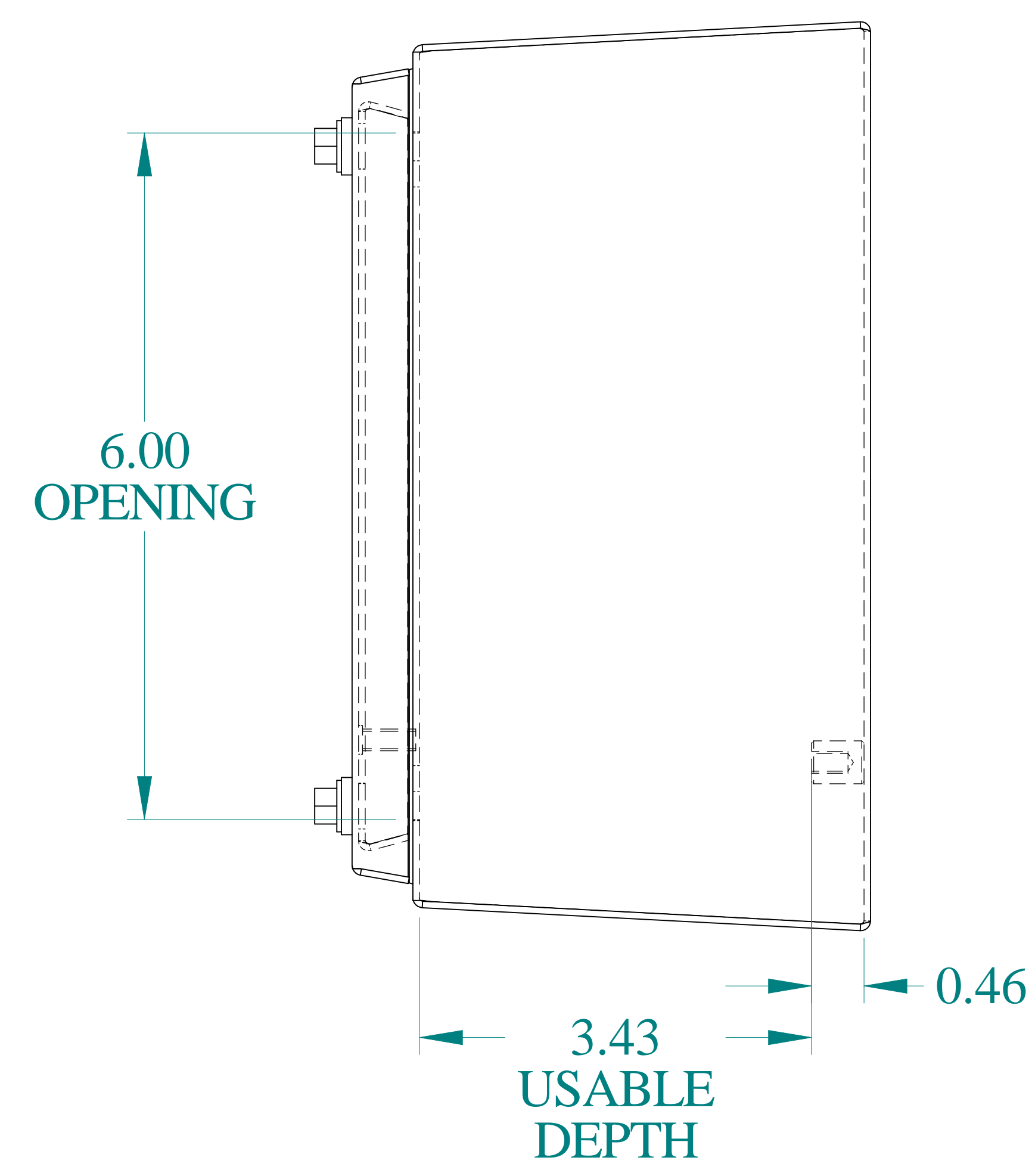
SIDE VIEW
