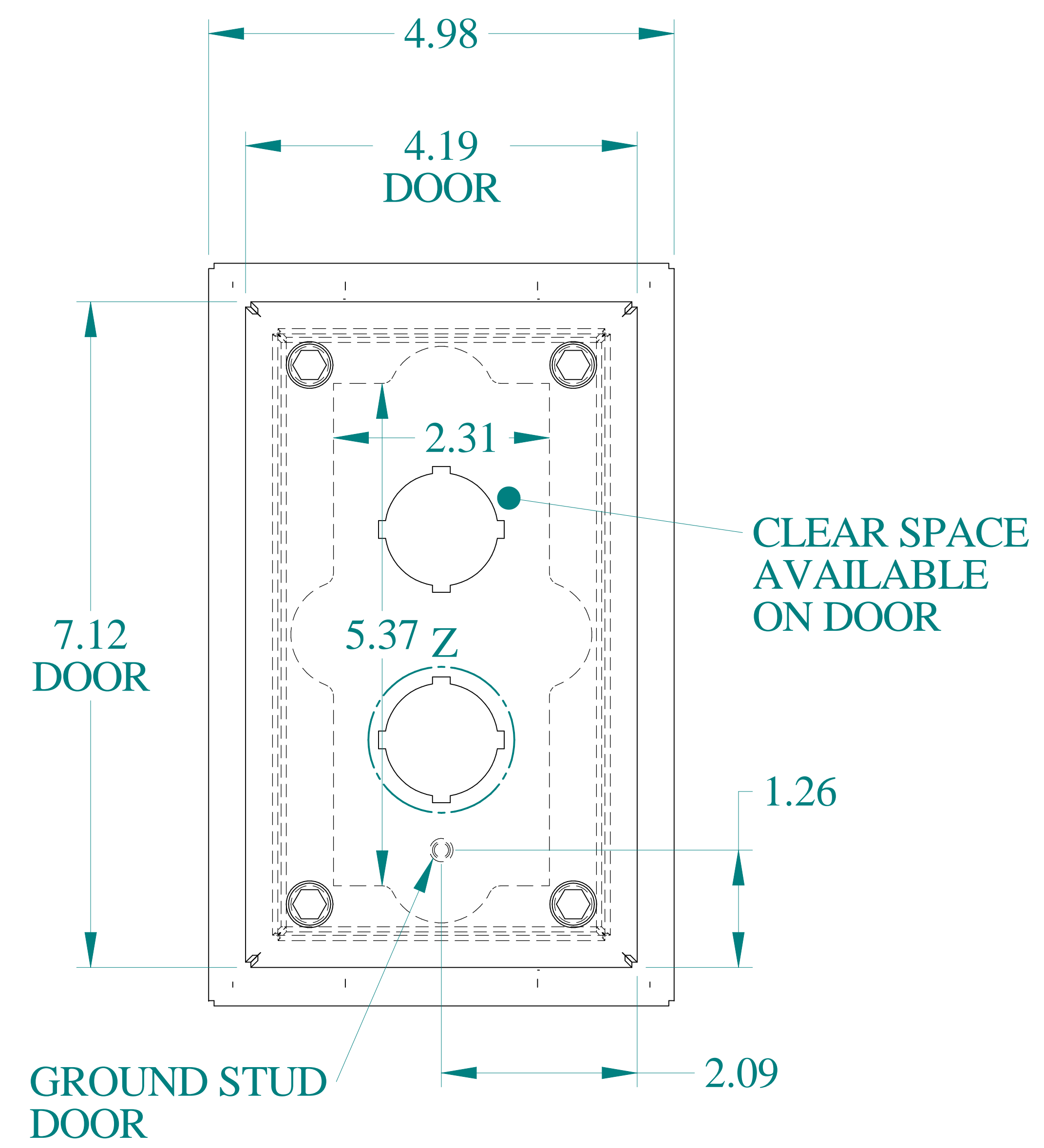
TOP VIEW
