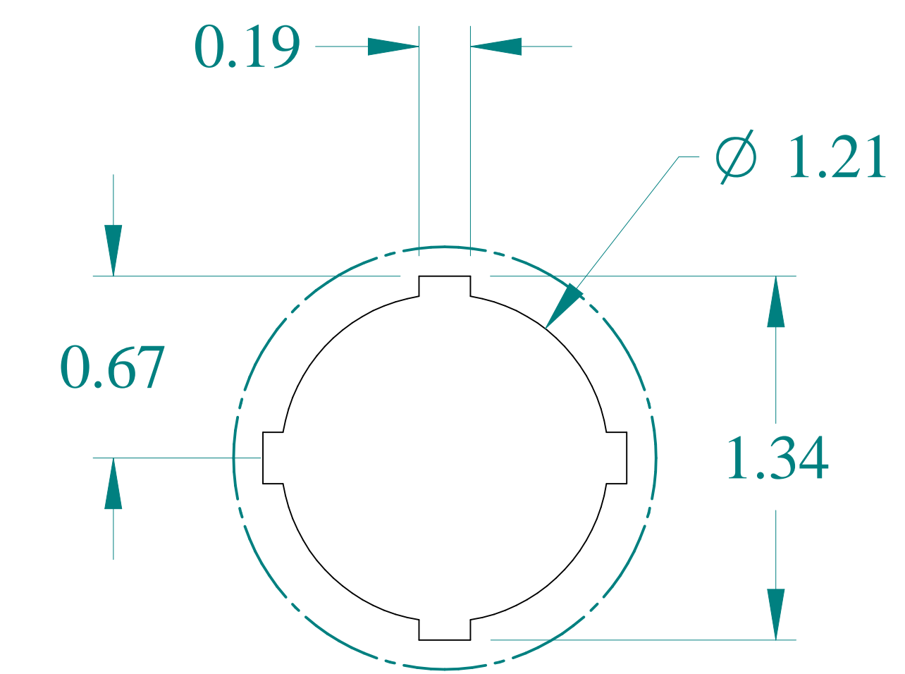
DETAIL Z
