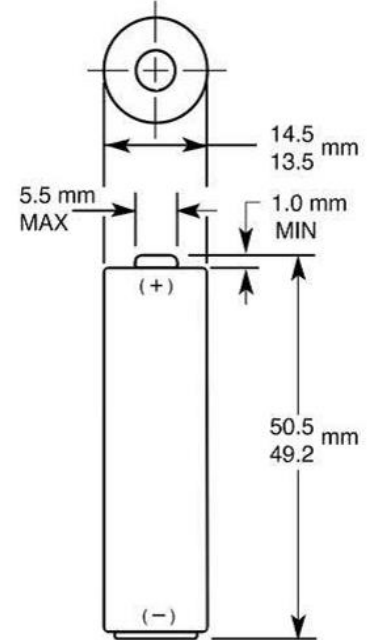
Dimensions shown are IEC standards
