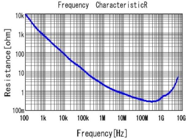
GCM155L81H102KA37 R DCOV, 25degC
