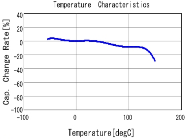
■ GCM155L81H102KA37 C-Temp. capchange, DCO. 0V, AC1.0V rm
