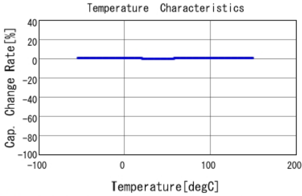
■ GCM1555G1H220JA16 C-Temp. capchange, DCOV, AC1Vrms
