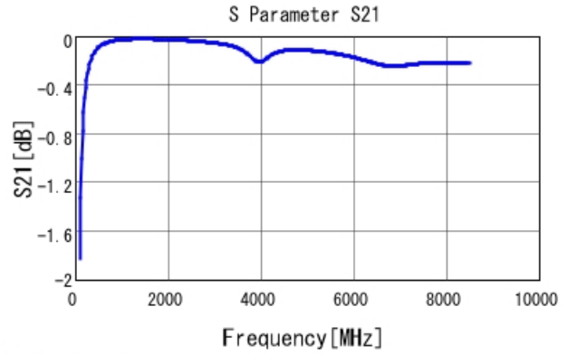
■ GCM1555G1H220JA16 S21 DCOV, 25degC
