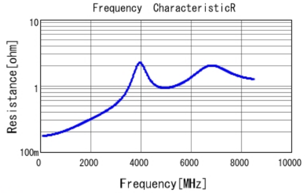
GCM1555G1H220JA16 R DC0V, 25degC
