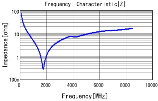
GCM1555G1H220JA16 |Z| DC0V, 25degC
