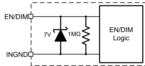
Figure 3: Internal EN/DIM Circuit
