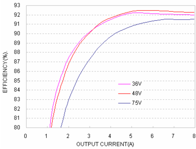
Figure 1: Efficiency vs. load current for 8A, minimum, nominal, and maximum input voltage at 25°C
