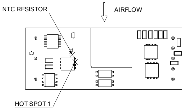
Figure 19: * Hot spot 1 & NTC resistor temperature measured points
