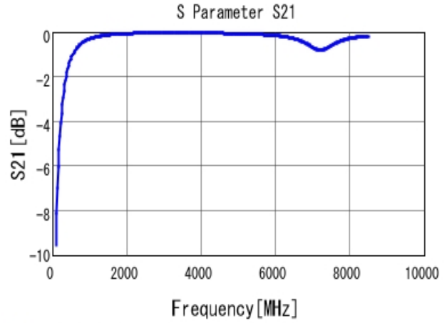
■ GCM1555C1H5R6CA16 S21 DCOV, 25degC
