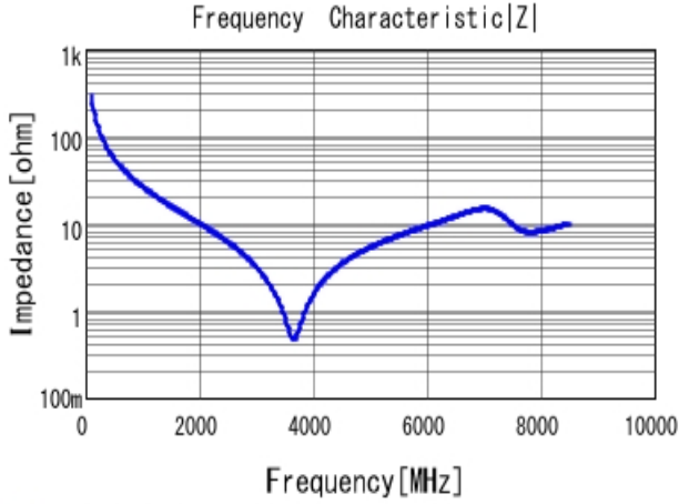
■ GCM1555C1H5R6CA16 |Z| DC0V, 25degC
