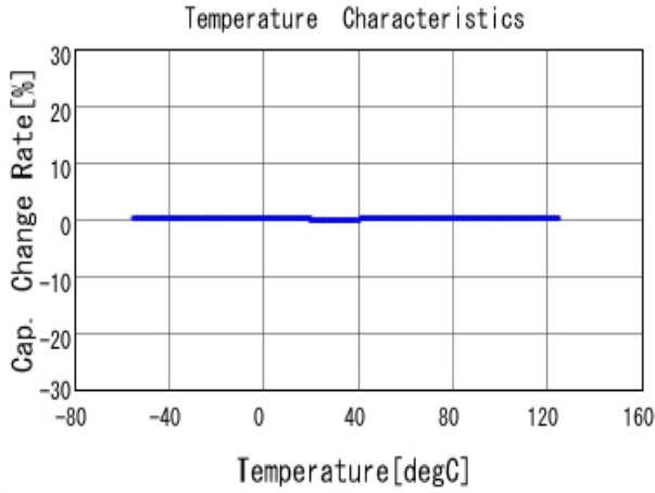
■ GCM1555C1H5R6CA16 C-Temp. capchange, DCOV, AC1Vrms
