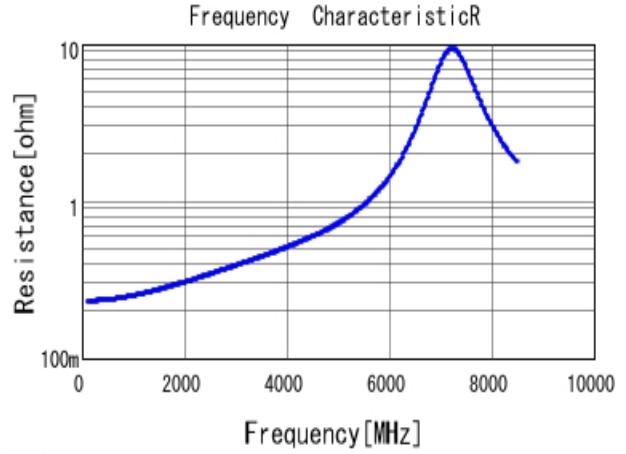
■ GCM1555C1H5R6CA16 R DC0V, 25degC
