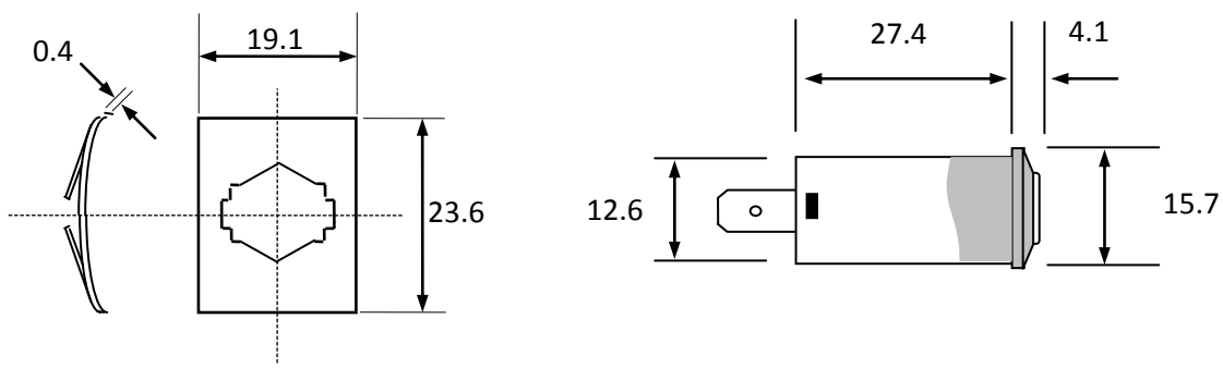
Spire nut for panel fixing
