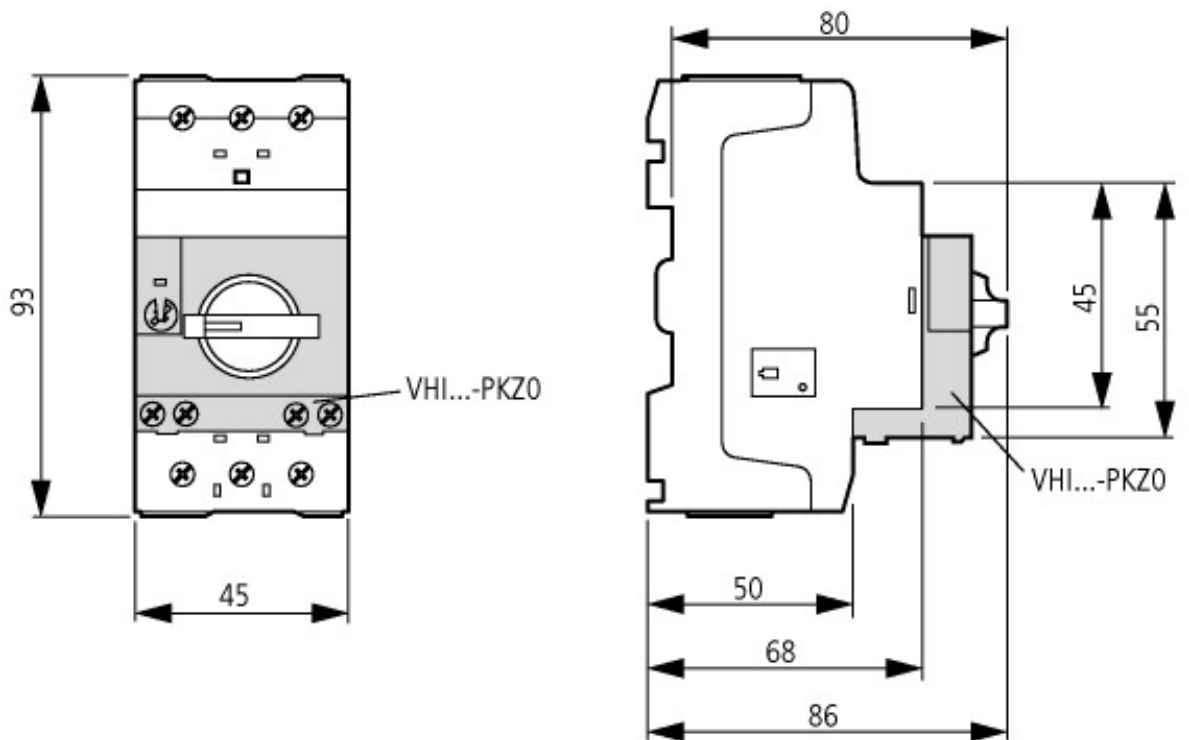
Motor-protective circuit-breakers with early-make auxiliary contacts PKZM0-...+VHI-...-PKZ0
