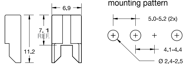
Dimensions in mm / Maße in mm
