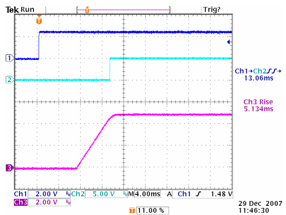
Figure 18: Turn on delay time at 12Vin, 5.0V/40A out (4mS/div) Ch1: Enable, Ch2: PG, Ch3: Vo
