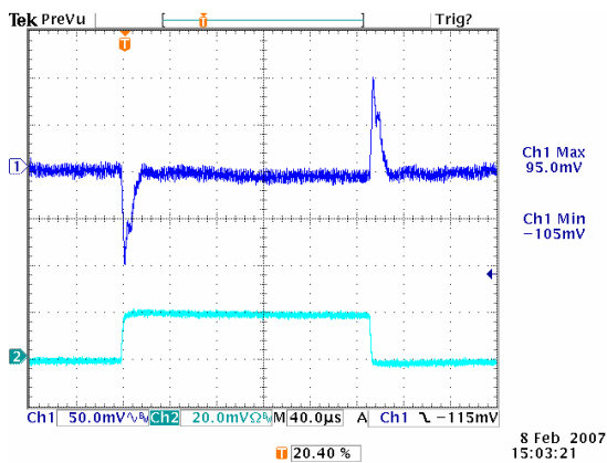
Figure 23: Transient Response at 12Vin, 3.3V/40A out (40uS/div) Ch1: Vo, Ch2: Io, 10A/div
