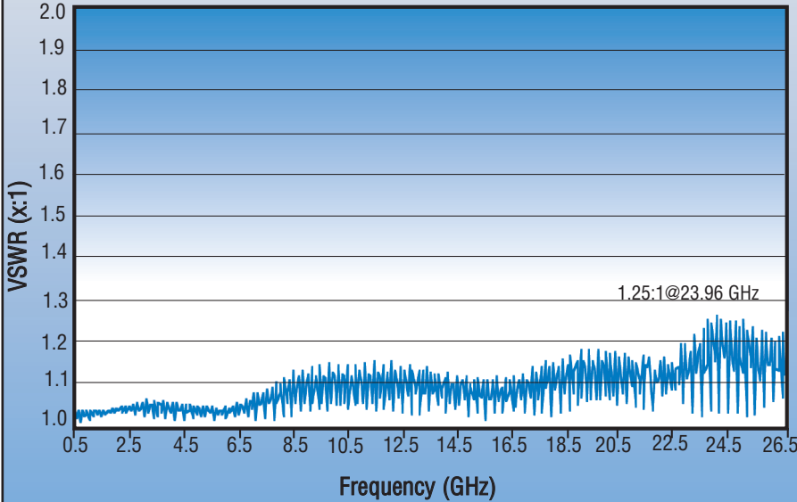
(26.5 GHz SMA Male/SMA Male, 3 ft long)
