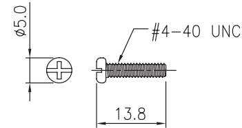
SCREW *2PCS
