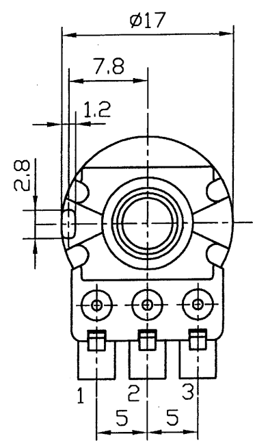
TERMINAL DETAIL
