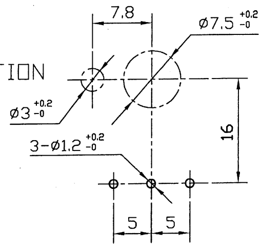
MOUNTING HOLE DETAIL (VIEWPOINT OF SHAFT)
