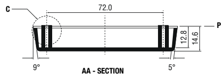
AA - SECTION
