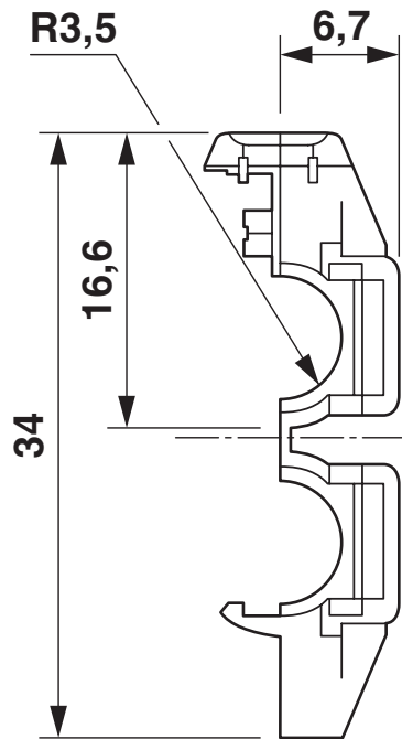
RJ45-Knickschutztülle
