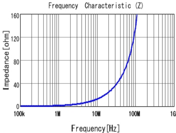
DFE252010F-R22M |Z|
