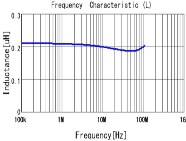
DFE252010F-R22M L
