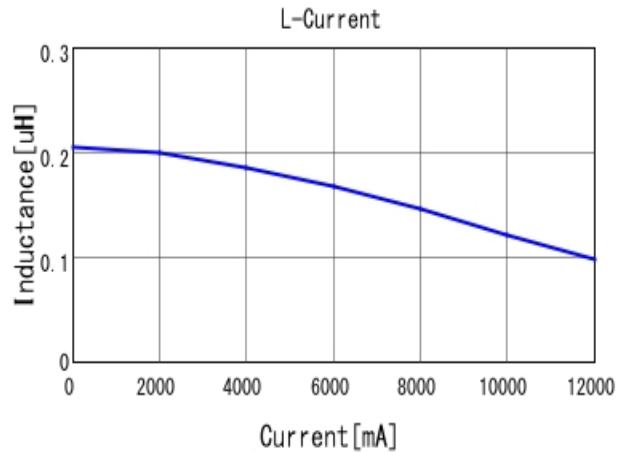
DFE252010F-R22M L-Current 20degC
