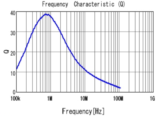
DFE252010F-R22M Q
