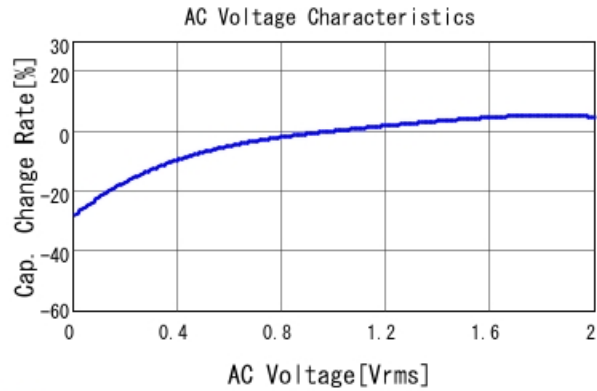
■ GRM188Z71C475KE21 C-AC Voltage capchange, DCOV, 25.0d
