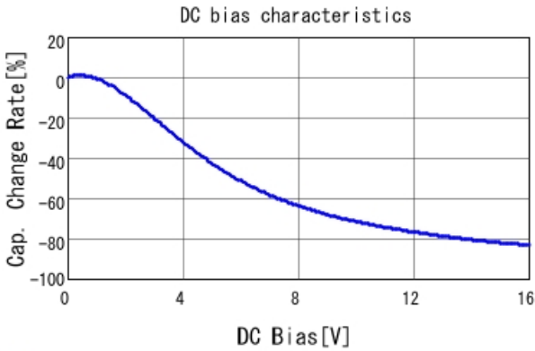
■ GRM188Z71C475KE21 C-DC bias capchange, 25.0degC, AC1V
