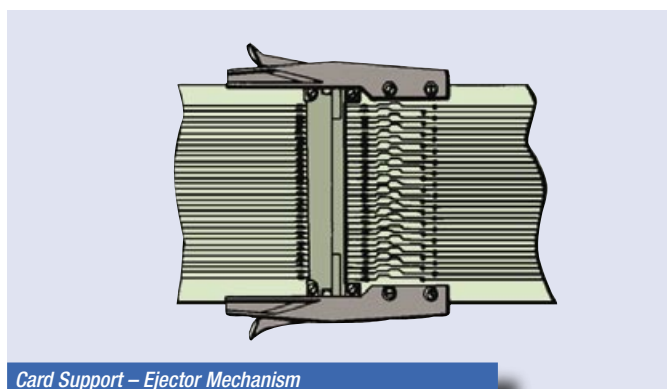
Card Support – Ejector Mechanism
