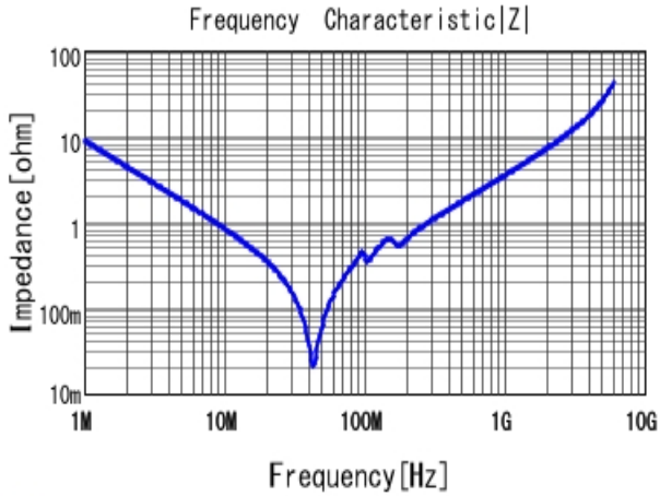
■ GRM3195C1H183JA01 |Z| DCOV, 25degC
