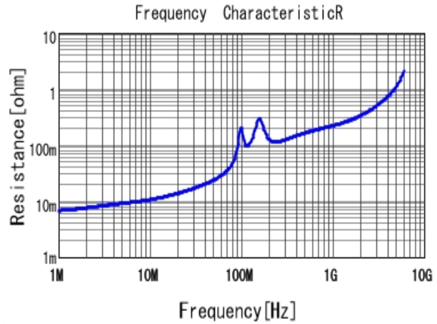
■ GRM3195C1H183JA01 R DCOV, 25degC
