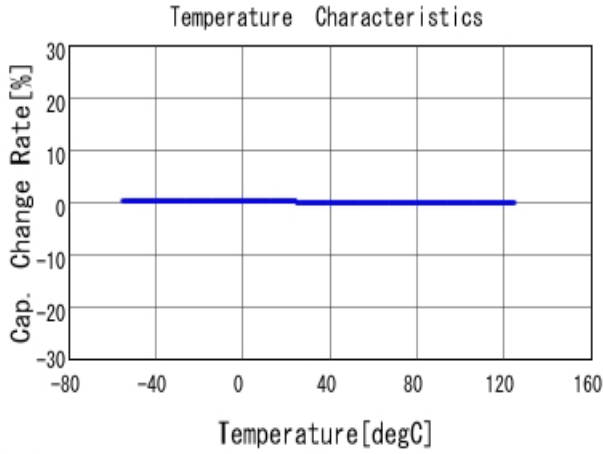
■ GRM3195C1H183JA01 C-Temp. capchange, DCOV, AC1Vrms
