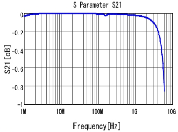
■ GRM3195C1H183JA01 S21 DCOV, 25degC
