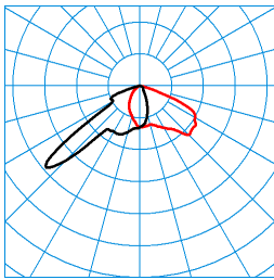
LIQ 70N-FL1L/6800-740 8G1 ET(CLO end value) TX278259 ■ C0 - C180 ■ C90 - C270 DIN 5040: A40 UTE: 1,00 F CEN Flux Code: 43 84 100 100 100
