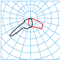
LIQ 70N-FL1L/6800-740 8G1 ET(CLO initial value) TX278239 ■ C0 - C180 ■ C90 - C270 DIN 5040: A40 UTE: 1,00 F CEN Flux Code: 43 84 100 100 100
