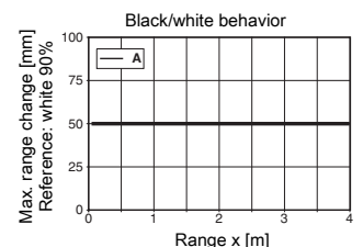
A 4% ... 90% diffuse reflection
