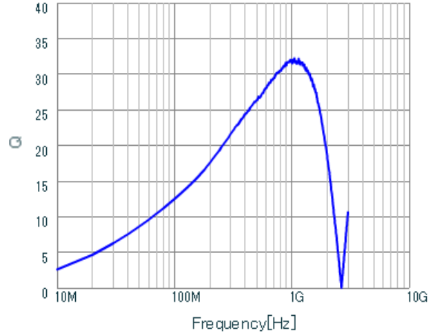
LQP03HQ33NJ02 Q.
