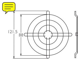
LZ22N Welded steel guard, bright zinc. 8xxx series fans
