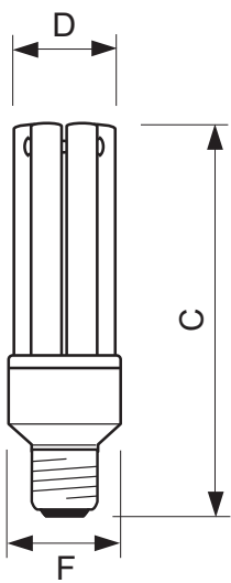
MASTER PLE-R 15W/827 E27 220-240V 1CT
