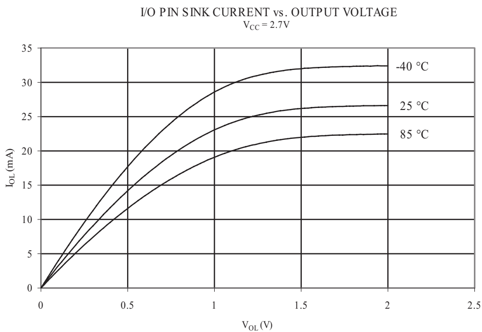
Figure 33-25 I/O Pin Sink Current vs. Output Voltage, V_{CC} = 2.7V
