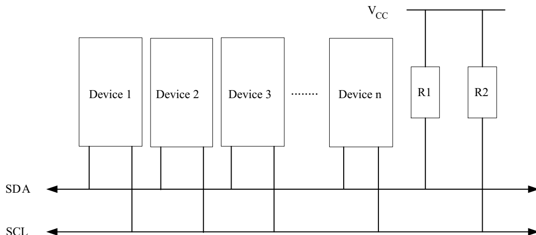
Figure 26-2 TWI Bus Interconnection
