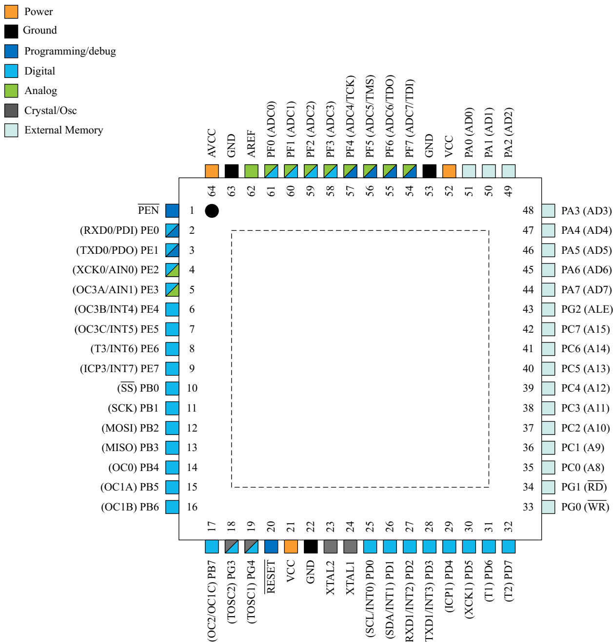
Figure 6-1 Pinout ATmega128A
