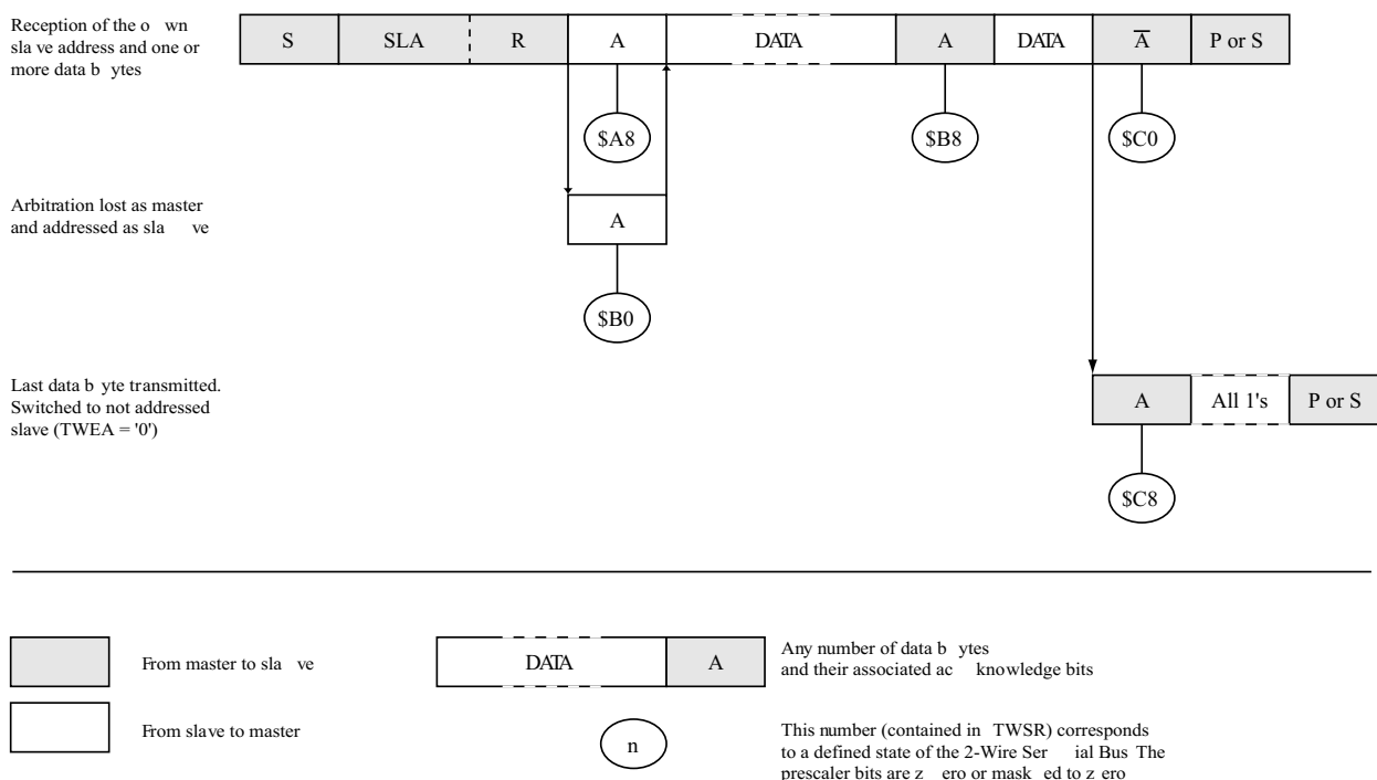
Figure 26-18 Formats and States in the Slave Transmitter Mode
