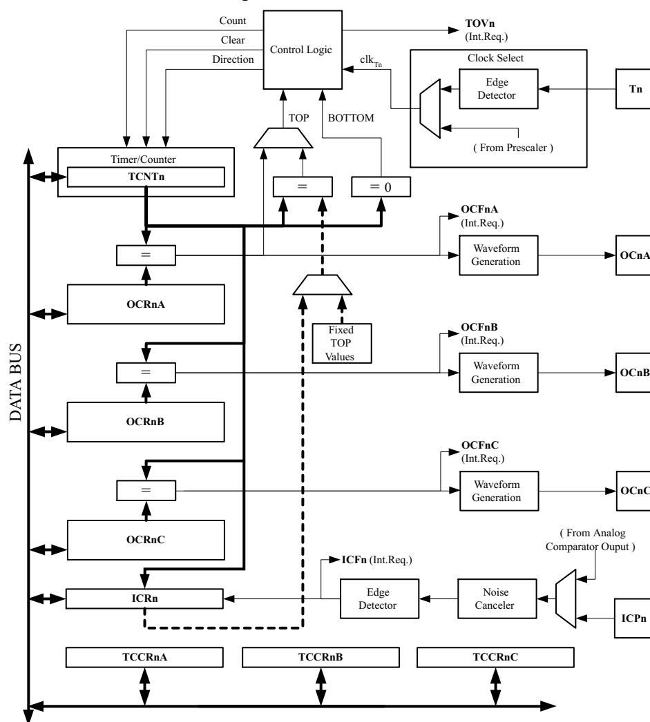
Figure 20-1 16-bit Timer/Counter Block Diagram (1)
