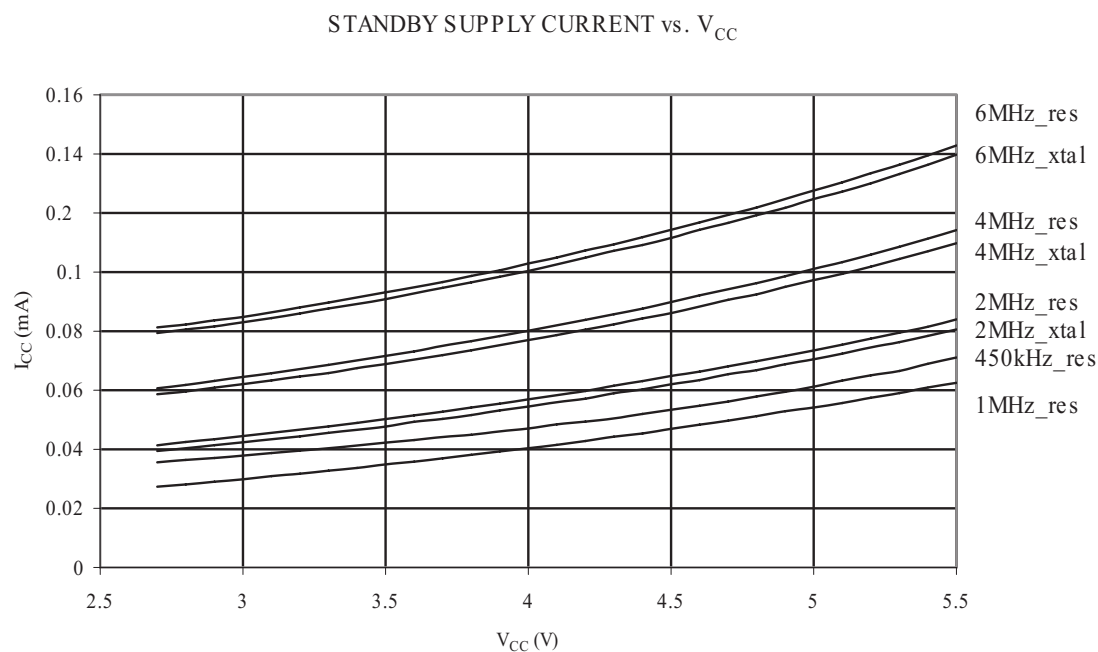
Figure 33-18 Standby Supply Current vs. V_{CC} ,
