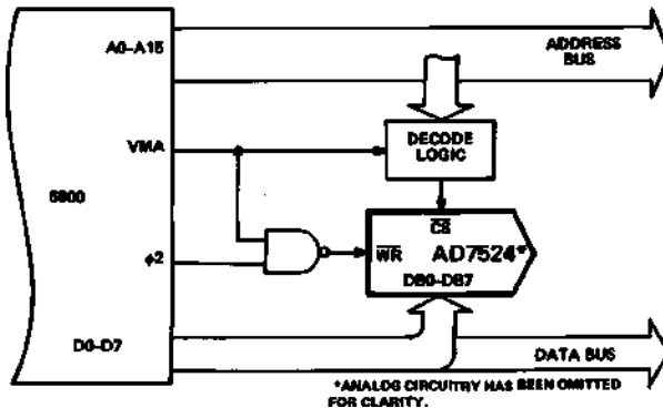
Figure 7. AD7524/MC6800 Interface
