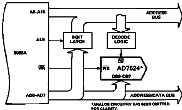
Figure 6. AD7524/8085A Interface
